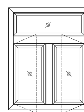
DOUBLE SHUTTER OUTSIDE OPENING SIDE HUNG + TOP FIX WINDOW
