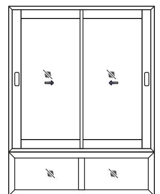
2T+2G SHUTTER SLIDING + BOTTOM FIXED WITH CENTER MULLION WINDOW
