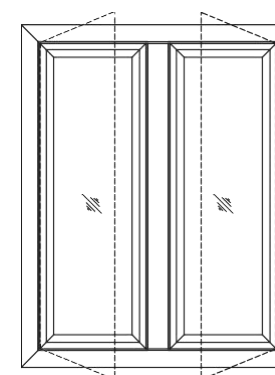
DOUBLE SHUTTER OUTSIDE OPENING SIDE HUNG WINDOW
